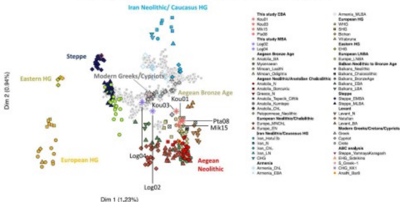
MDS of six Aegean genomes alongside published modern and ancient Eurasian populations
